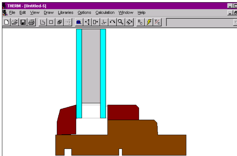
Figure 8-35. The glazing system from WINDOW has been inserted into the frame components.
