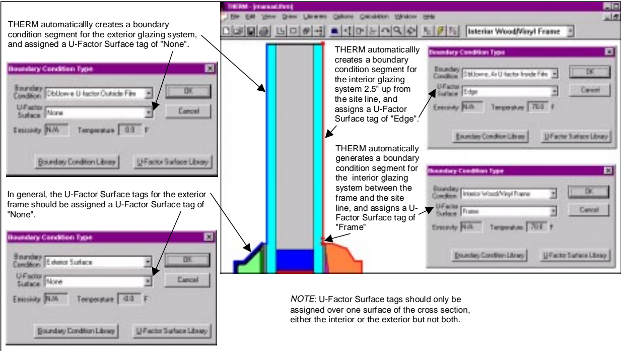
Figure 6-6. Assigning U-Factor Surface tags to different boundary segments. THERM automatically makes two boundary segments on the interior surface of the glazing system, one from the frame to the sight line (with a U-Factor Surface tag of "Frame") and one from the sight line up to 2.5" of the glass (with a U-Factor Surface tag of "Edge").
