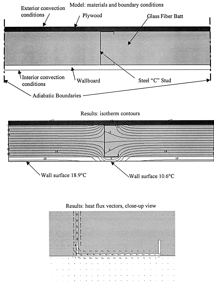
Figure 3 THERM model of an “insulated” steel stud wall: cross section (top), results—isotherms (middle), and results—heat flux vectors (bottom).
